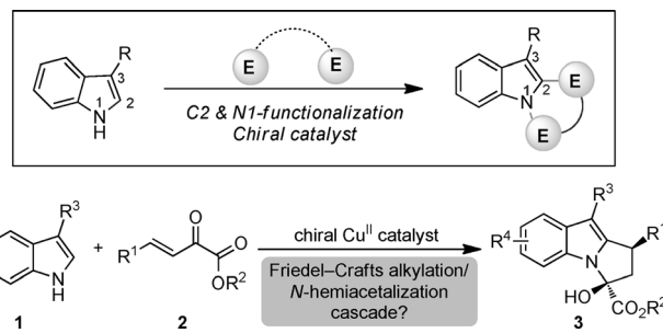
Scheme 2. Conceptual basis for the enantioselective Friedel–Crafts alkylation/ N -hemiacetalization cascade reaction with indoles.
