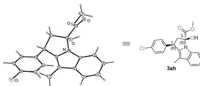
Figure 1. X-ray crystal structure of compound 3ah . [14] Thermal ellipsoids set at 30% probability.
