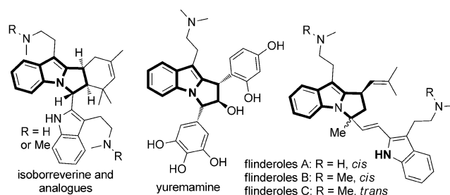
Scheme 1. Representative natural products based on 1 H -pyrrolo[1,2- a ]indole.
